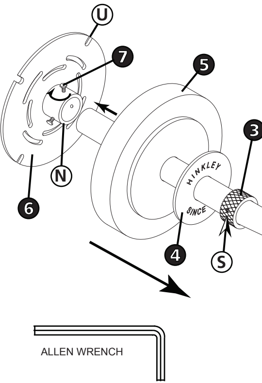
DRAWING 2 - ASSEMBLY
