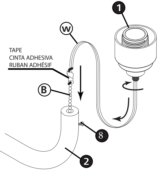
DRAWING 1 - ASSEMBLY
