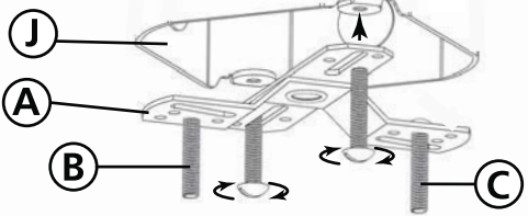
Drawing 2 - Fixture Mounting
