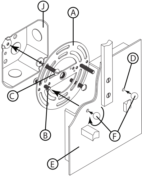
DRAWING 1 - MOUNTING
