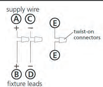
Drawing 3 – Post-Mount
