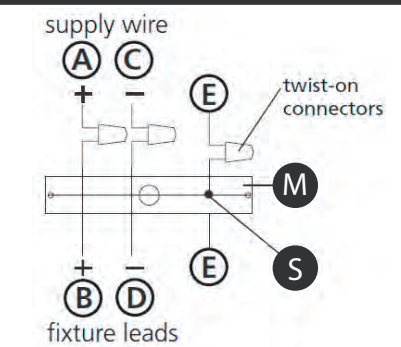
Drawing 3 – Post-Mount
