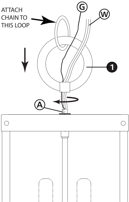
DRAWING 1 - ASSEMBLY
