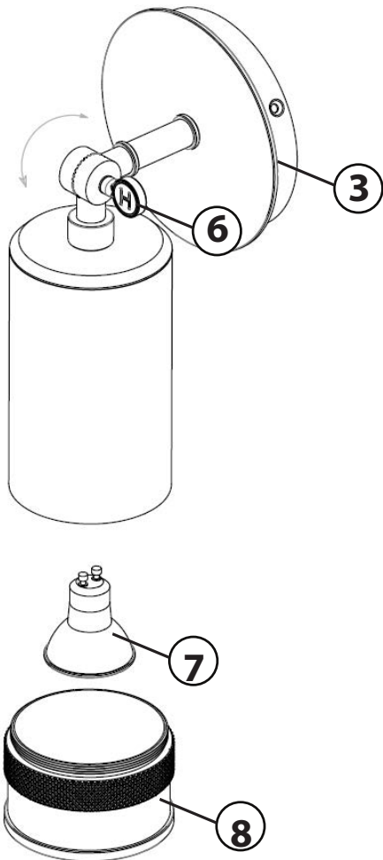
DRAWING 2 - Fixture Installation
