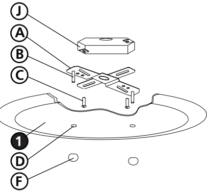
Drawing 3 - Glass Assembly
