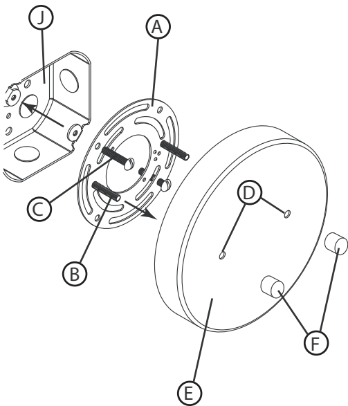
DRAWING 2- Glass install
